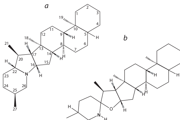
Fig. 1. Structures of two common SGA aglycones: a , solanidine; b , spirosolane.
