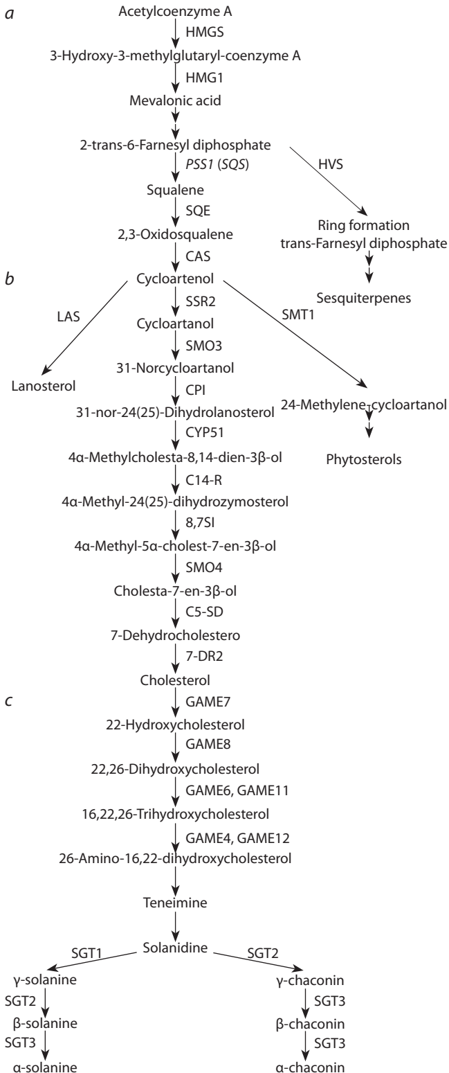
Fig. 4. Biosynthesis of steroidal glycoalkaloids (according to Itkin et al., 2013; Cárdenas et al., 2015; Sonawane et al., 2016).
