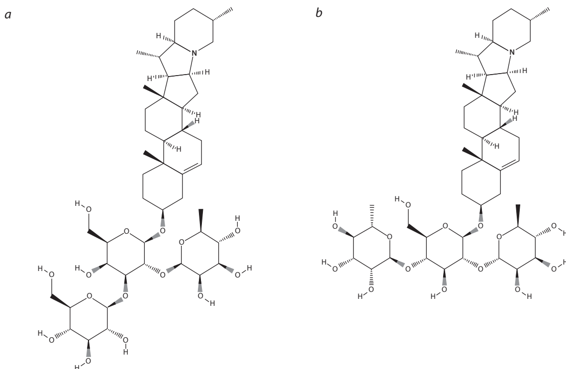
Fig. 3. Structures of glycoalkaloids involving the solanidine aglycone: a , \alpha -solanine; b , \alpha -chaconine.
