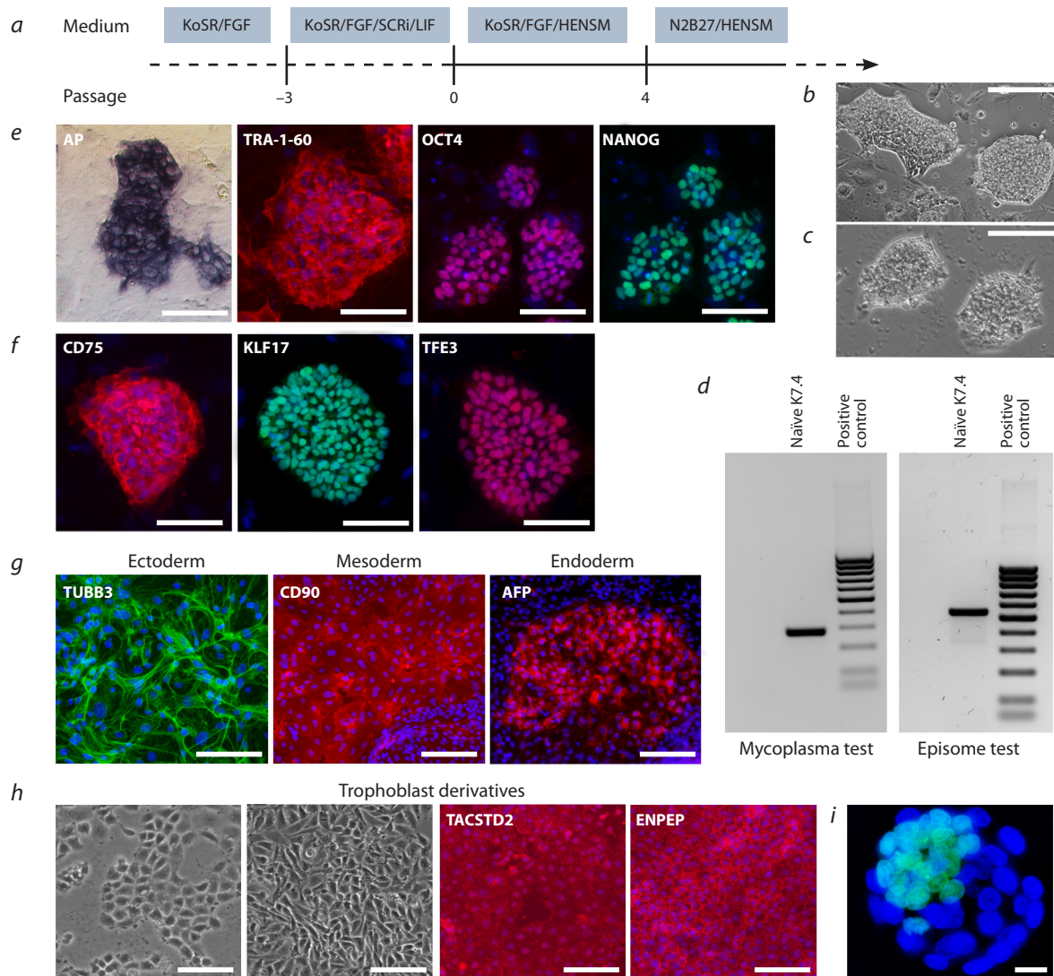
Fig. 1. K7-4Lf hiPSCs after induction of naïve pluripotency in HENSM medium.
