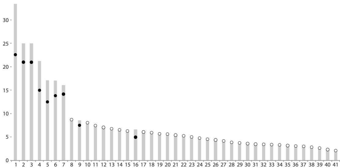
Fig. 3. SC idiogram of the pine grosbeak karyotype, excluding the GRC. The Y axis shows the average SC length in \mu\text{m} . The X axis shows bivalents ordered by decreasing size. Black circles indicate the location of monocentromeres, white circles indicate metapolycentromeres.
