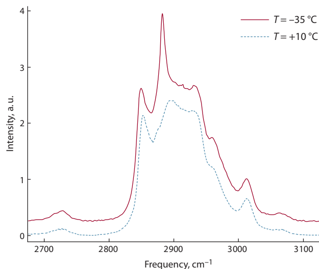
Fig. 4. Raman spectra measured from lipid drops of the cat embryo at various stages of the freezing process.
